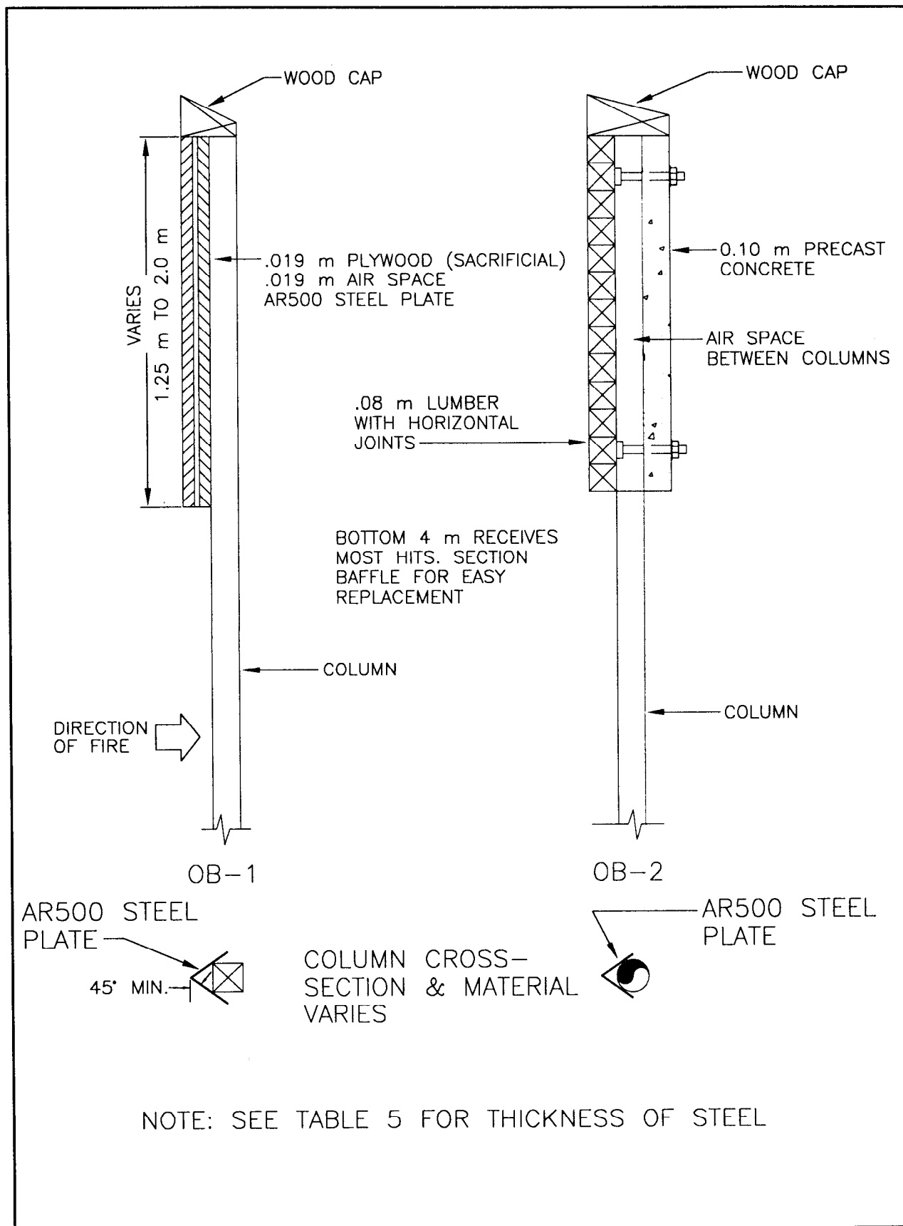
Figure 2.2-10 Overhead Baffle
