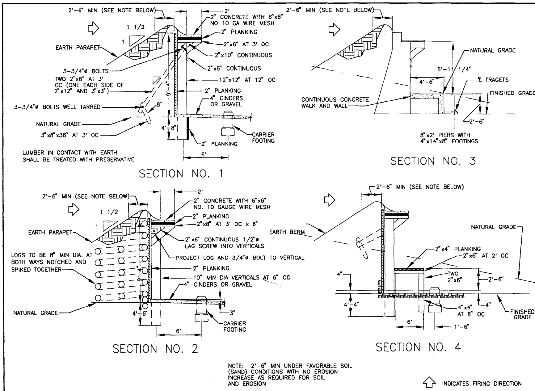
Figure 2.2-17 Alternate Target Butts
