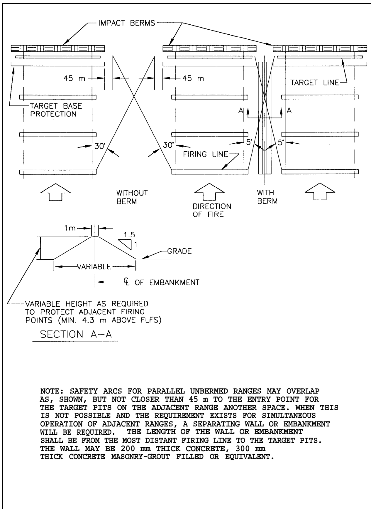
Figure 2.2-8 Parallel Ranges
